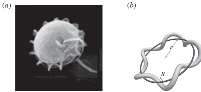
FIGURE 1. (a) A micrograph of the dinoflagellate, Pfisteria piscicida (courtesy of the Aquatic Botany Lab, NC State, USA). (b) A cylindrical ring that is helically wrapped around a baseline circle of radius r . The amplitude of the helix is R .
